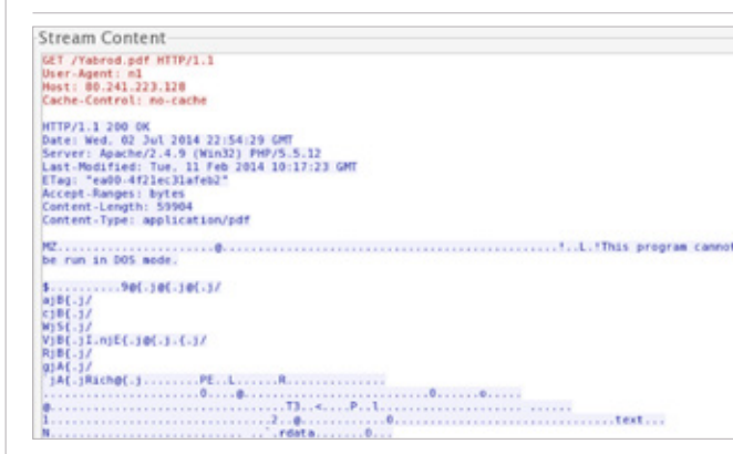
Figure 17: Downloading the file Yabrod.pdf
